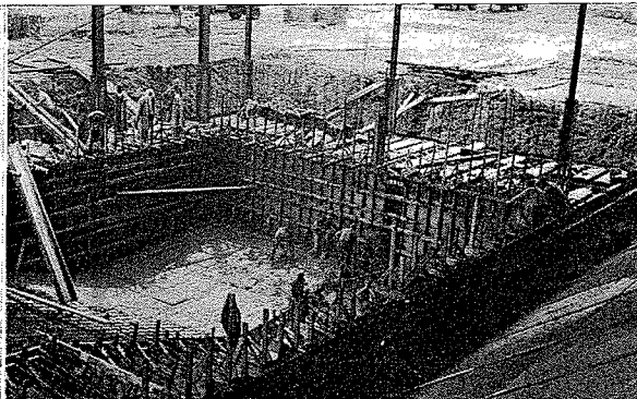
POOL BASIN has been poured in work of June 12-14. Deep section has 15-foot depth for future divers from high board.
