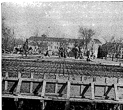
GYM FLOOR is poured in early stage of work. View is from south to north, length of varsity court.
